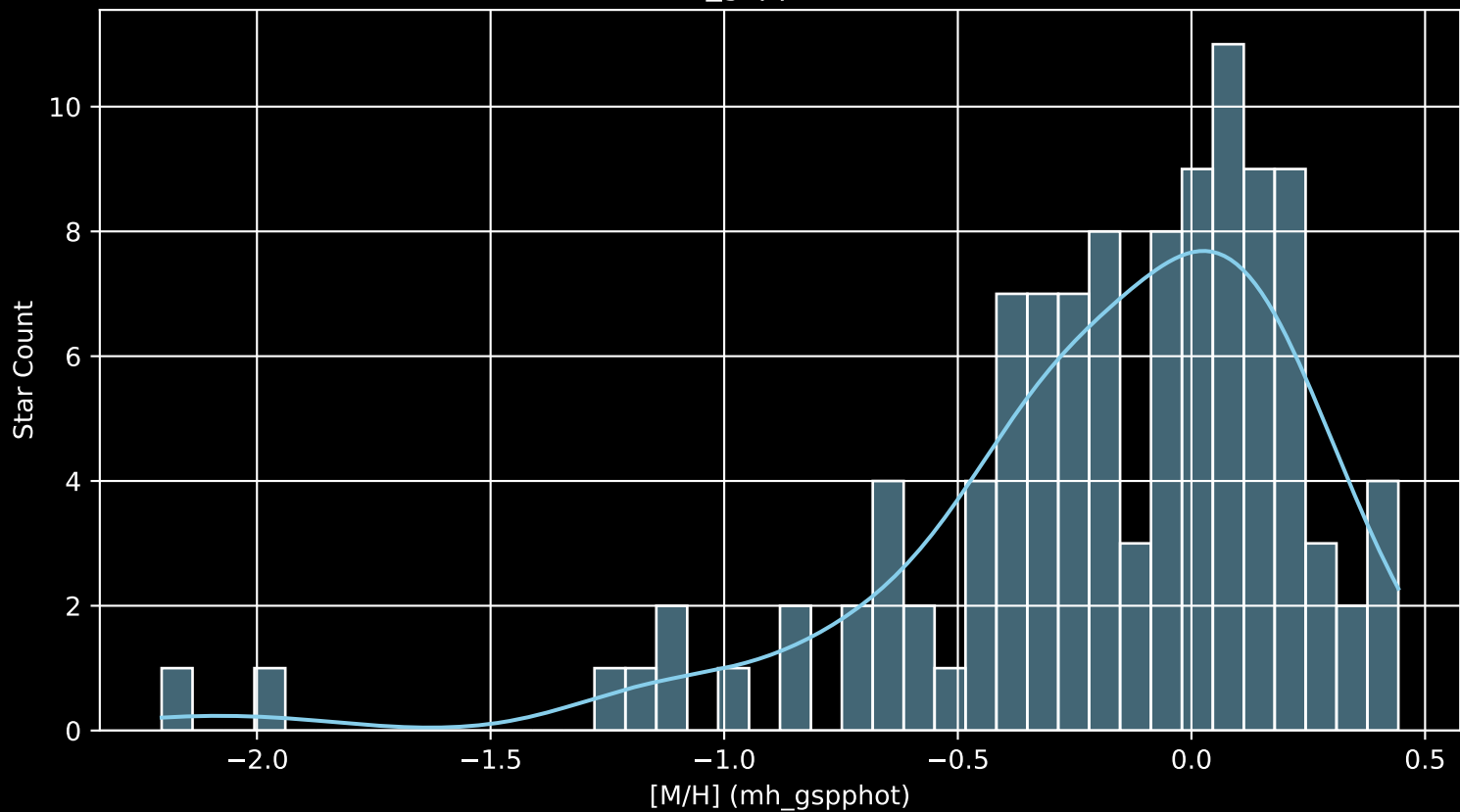
APOGEE DR17 Field: [LMC_VdS [M/H] (mh_gspphot) (n= 109)
