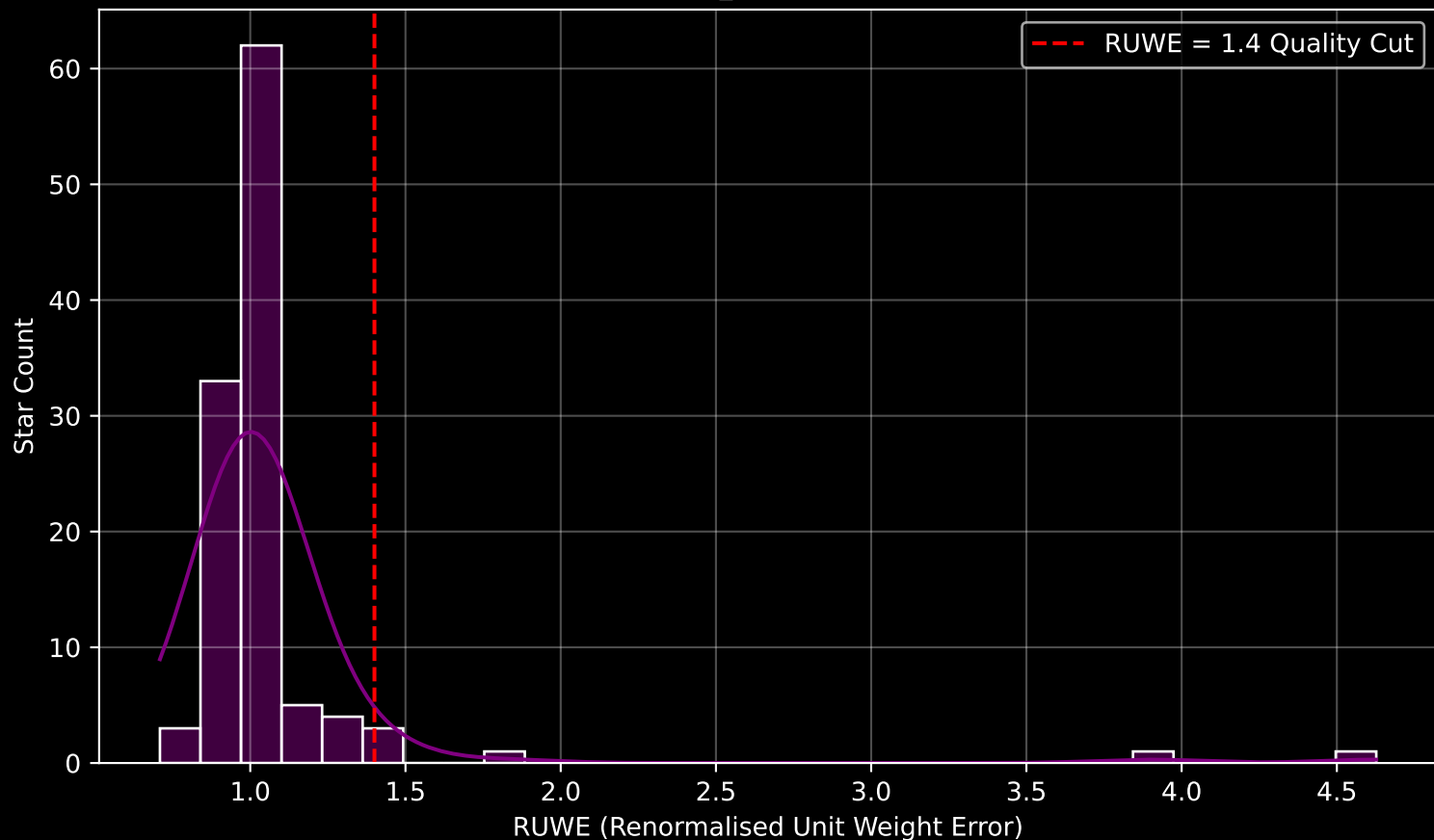
GAPOGEE DR17 Field [LMC_VdS] RUWE Distribution (n= 113)
