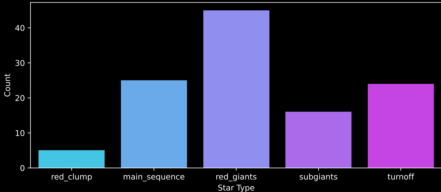
APOGEE DR17 Field: [LMC_VdS] Count plot of Star Type
