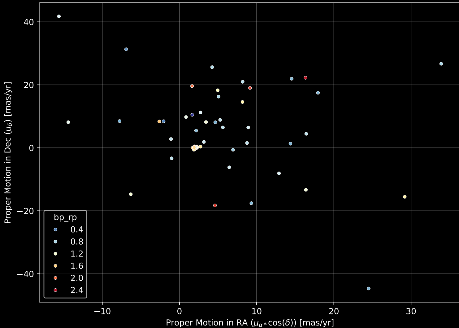
APOGEE DR17 Field: [LMC_VdS] Proper Motion Diagram (n= 115)
