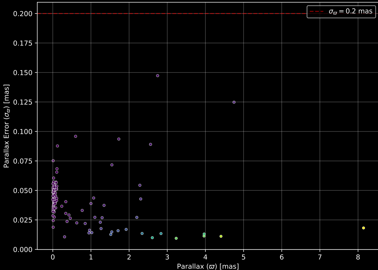
APOGEE DR17 Field: [LMC_VdS] Parallax Quality (n= 115)
